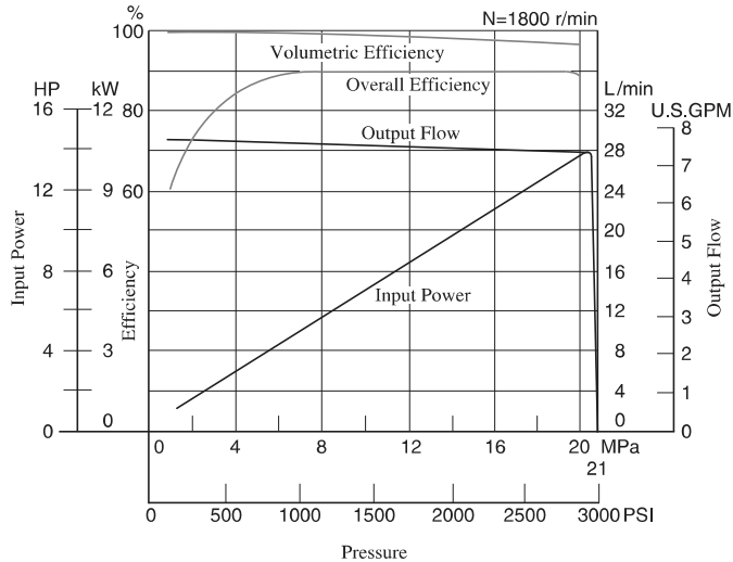
"A16" type performance characteristics
