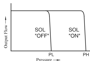
Performance Characteristics
