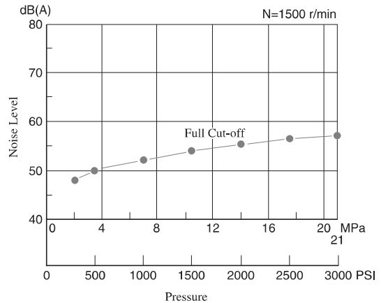
"A16" type noise level characteristics
