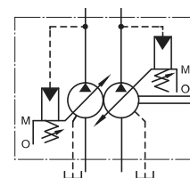
Graphic Symbol
