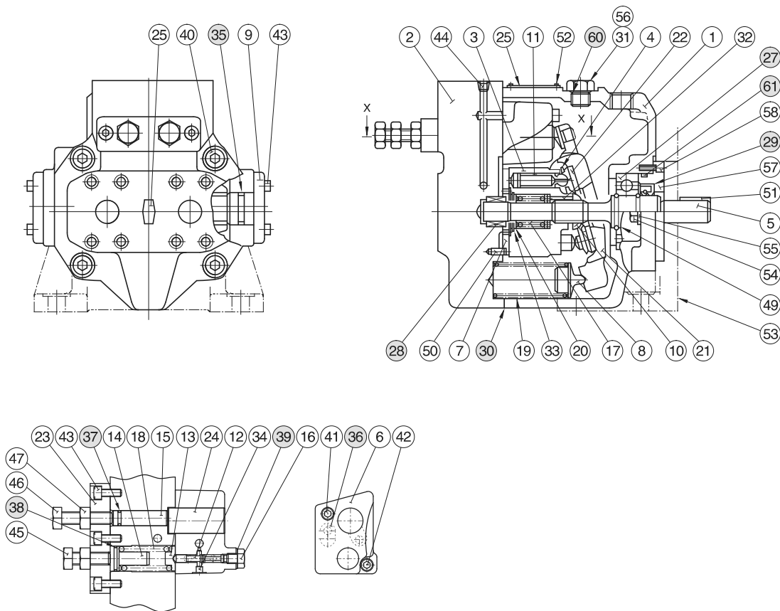
Section X-X
